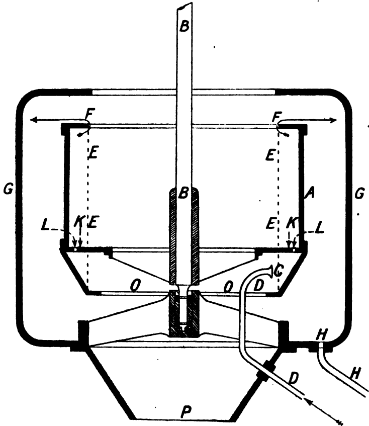
FIG. 22.—CENTRIFUGAL SUBSIDER
